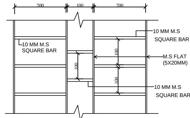
TYPICAL WINDOW AND VENTILATOR GRILL DETAIL
