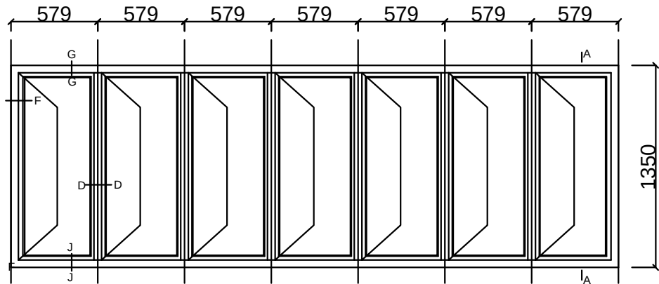
WINDOW TYPE W/V
