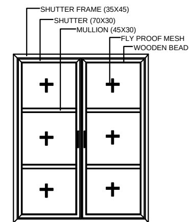
TYPICAL WINDOW AND VENTILATOR FLY PROOF DETAIL
