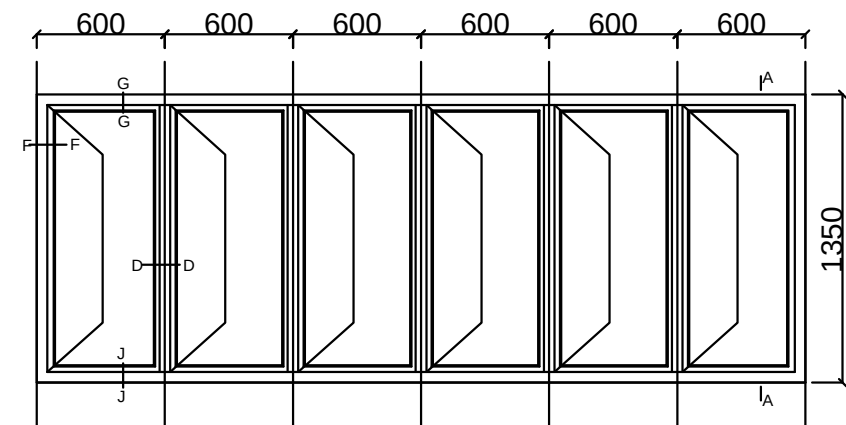
WINDOW TYPE W2/V2
