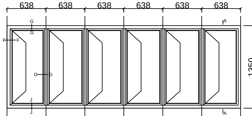
WINDOW TYPE W1/V1
